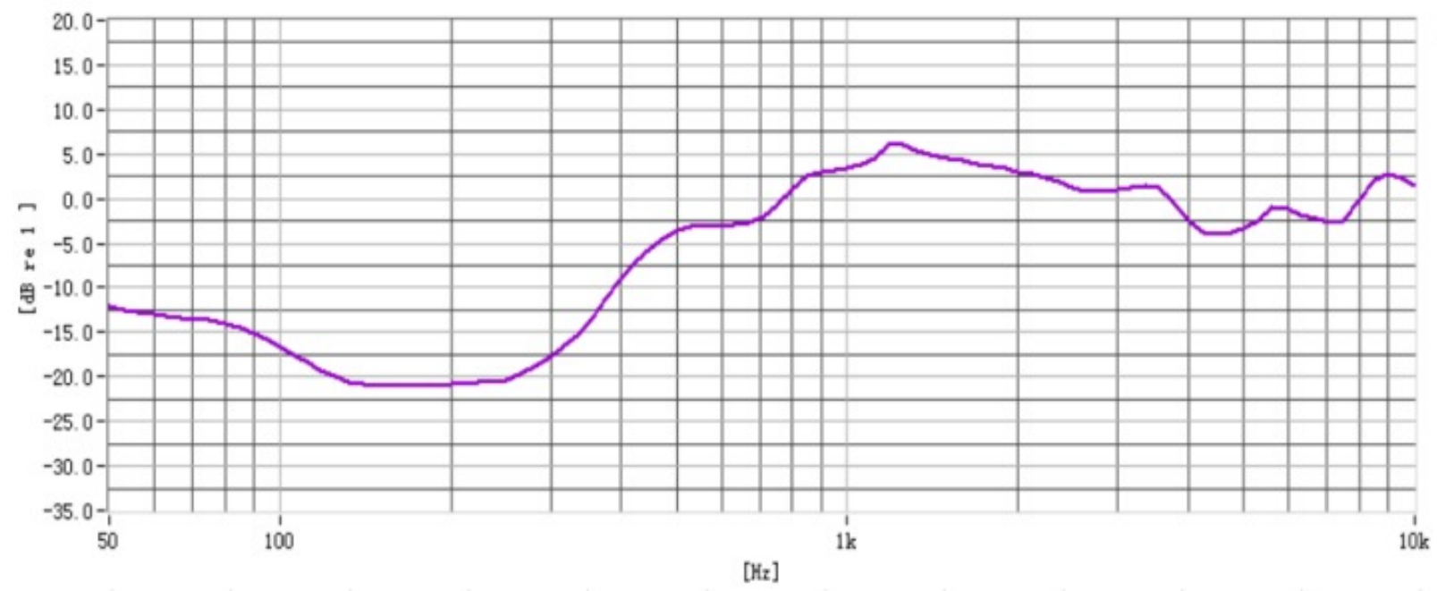
ANR Noise Cancelling Curve For Left Ear
