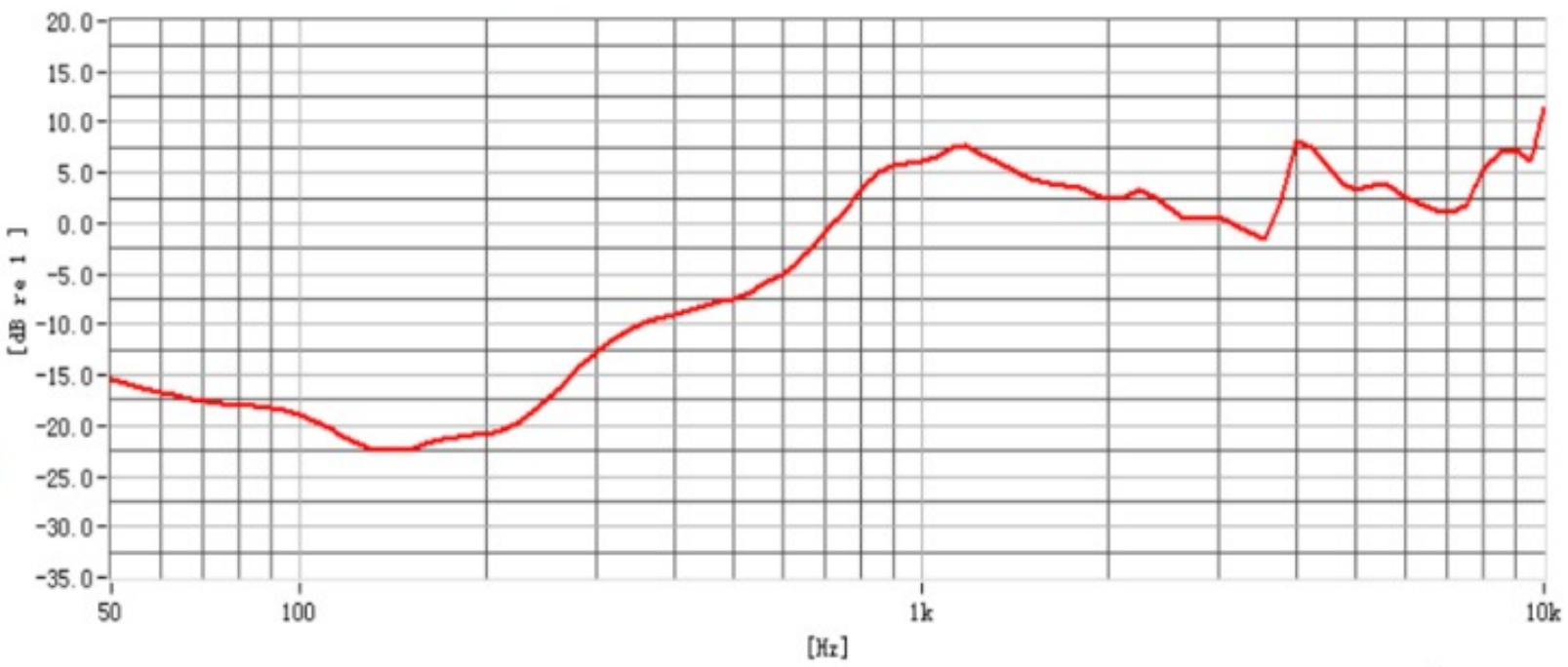
ANR Noise Cancelling For Left Ear
